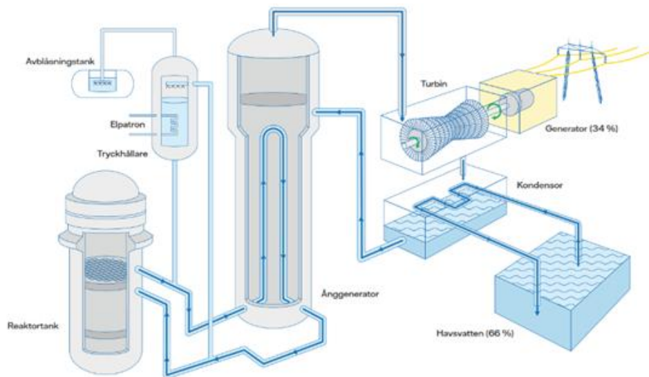
Figure 7. Schematic diagram of a pressurized water reactor. The numbers in the figure correspond to the energy distribution.
