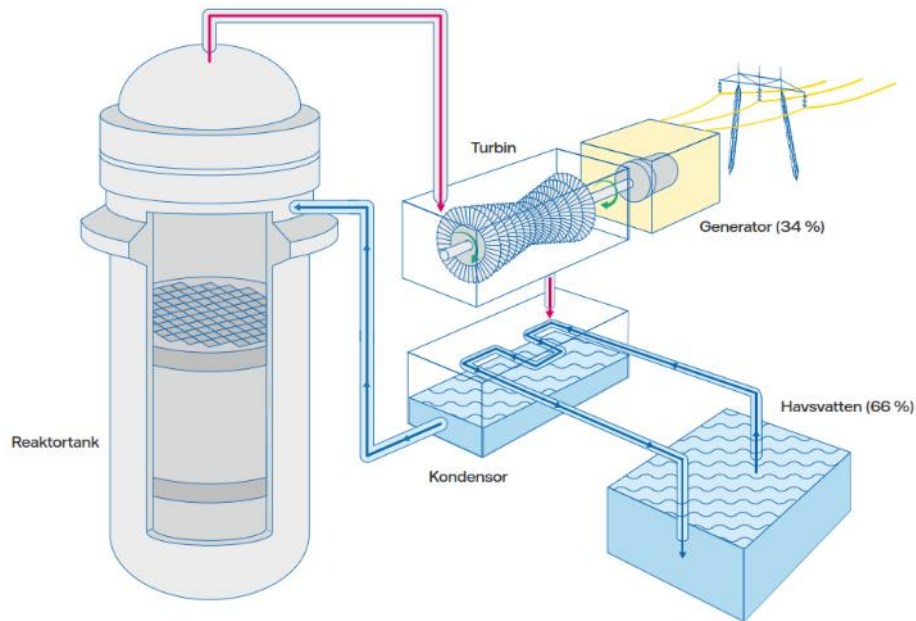
Figure 6. Schematic diagram of a boiling water reactor. The numbers in the figure correspond to the energy distribution.
