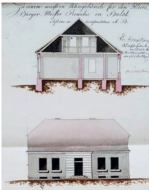
10. Projekt domu mieszkalnego dla mistrza Prosocha, Bielsk, 1805, APB, KWID, sygn. 2830, k. 415 Residential building design for Master Prosoch, Bielsk, 1805, State Archive in Białystok, War and Domain Office, ref. 2830, k. 415
