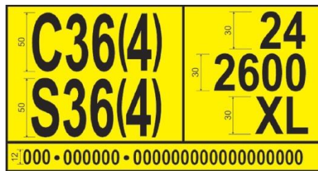
Figure 4.4 Yellow operational mark for swap bodies
