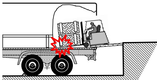
Figure 5.7 Grounding on down slope
