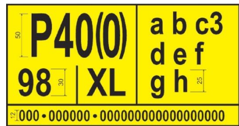
Figure 4.5 Yellow operational mark for trailers
