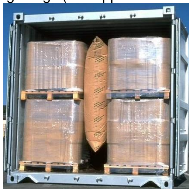
Figure 7.9 Gap filled with a central dunnage bag
