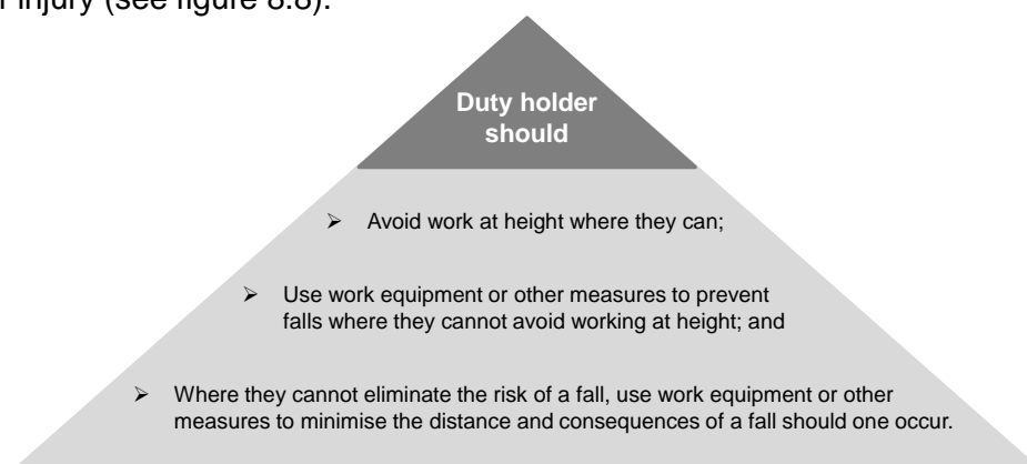
Figure 8.8 Regulations hierarchy
