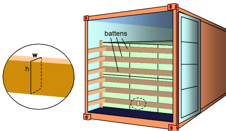
Figure 7.57 Transverse battens in an freight container
